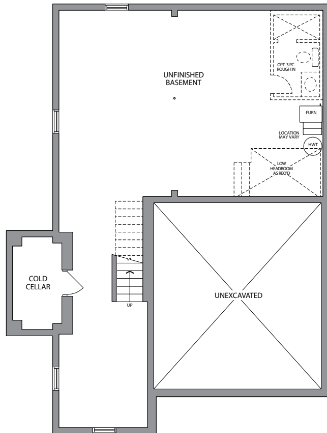
LOWER LEVEL ELEVATION A & B
