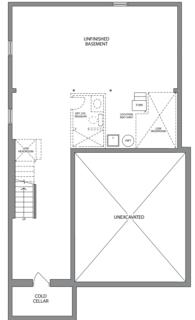
LOWER LEVEL ELEVATION C
