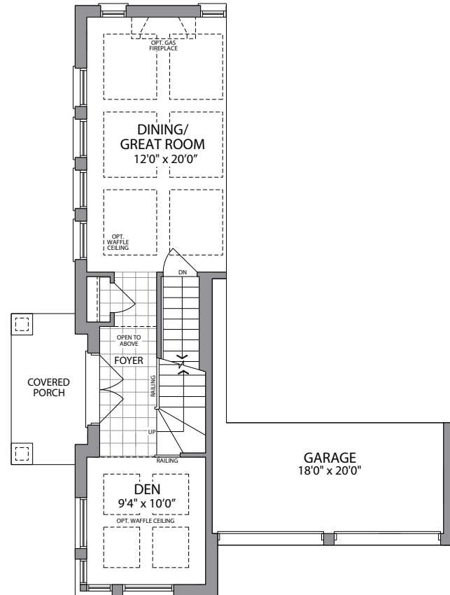
PARTIAL MAIN LEVEL
