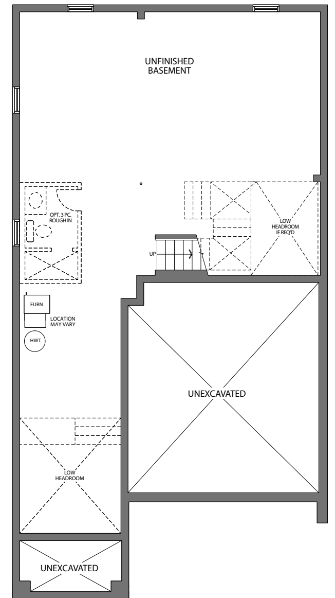
LOWER LEVEL ELEVATION D
