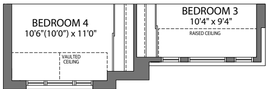
PARTIAL UPPER LEVEL ELEVATION B
