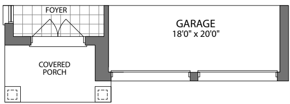
PARTIAL MAIN LEVEL ELEVATION B & C
